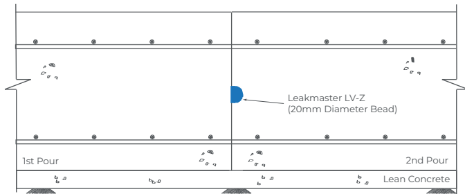
Application of Leakmaster LV-Z in Construction Joint of Wall or Slab
